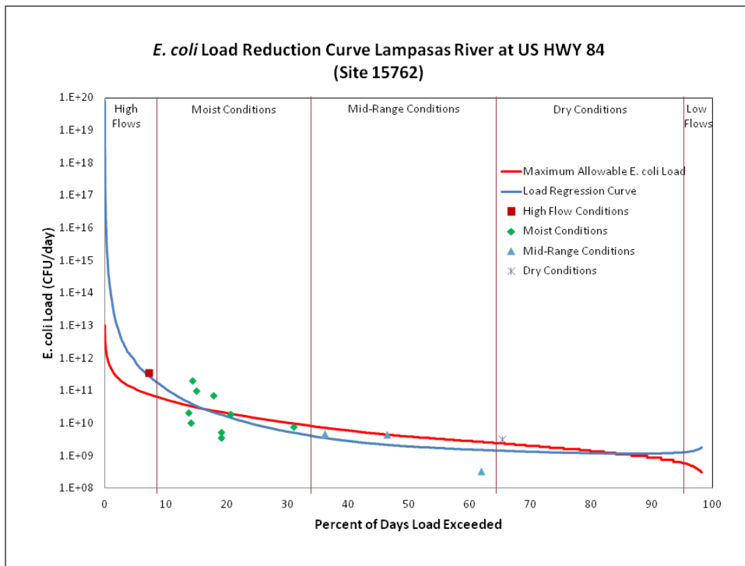
Figure 5.3 E. coli load duration curve for station 15762.
