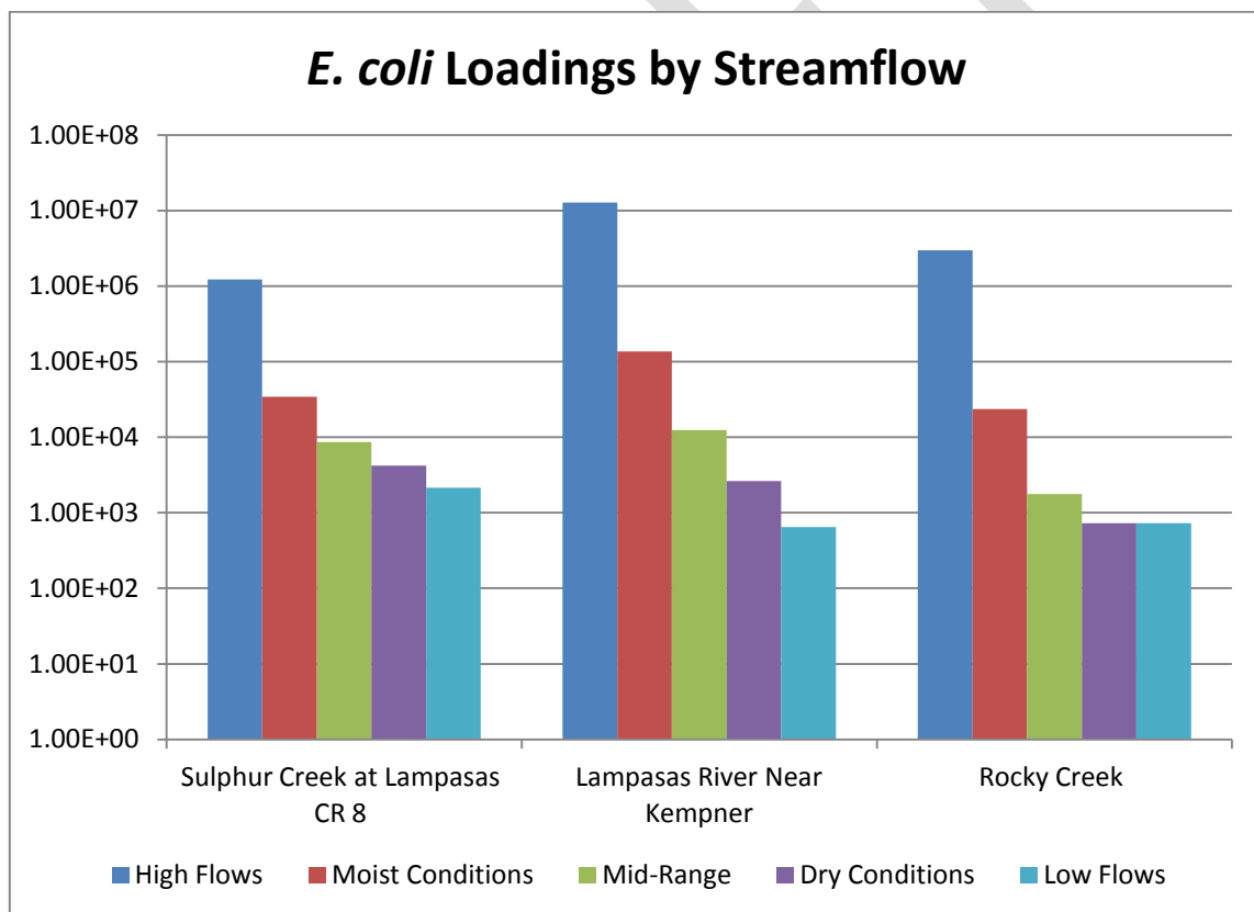
Figure 5.14 Estimated average annual E. coli loadings (billions of cfu) under different flow conditions at three water quality monitoring sites within the Lampasas River watershed.
