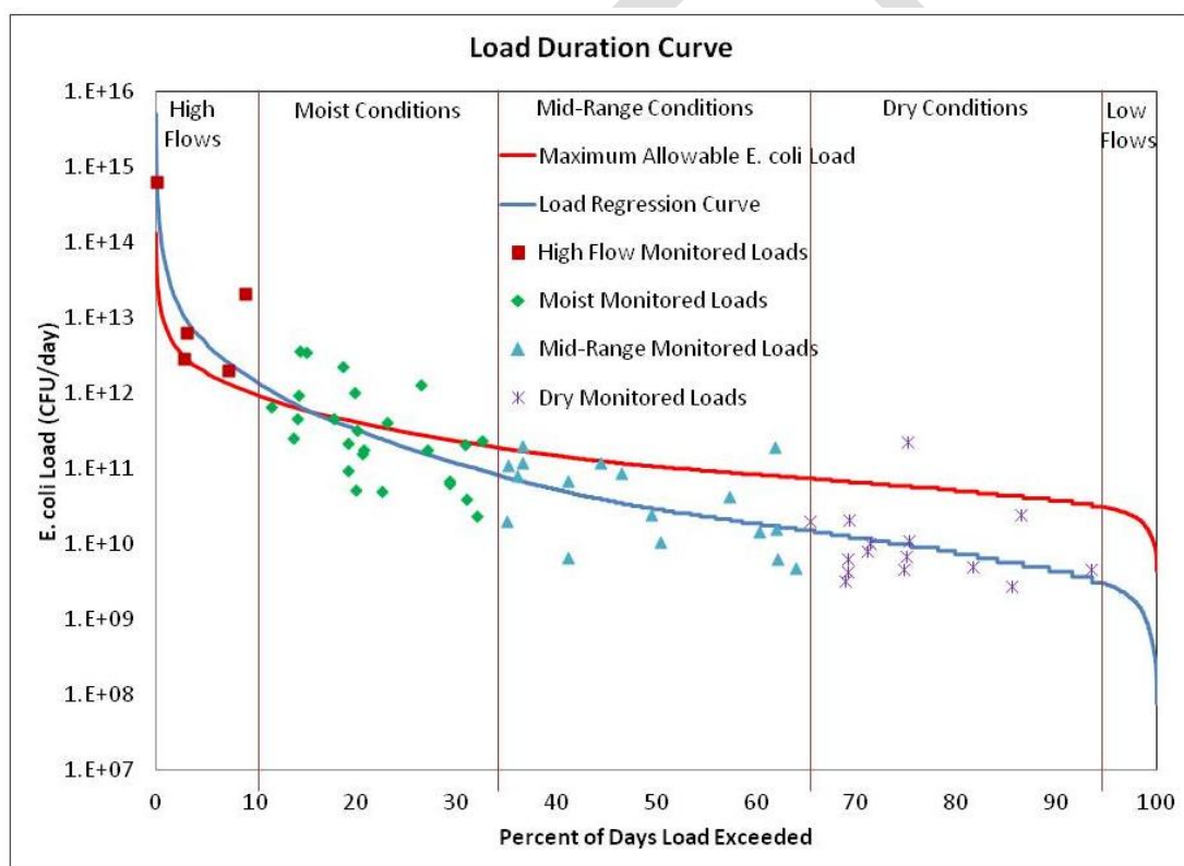
Figure 4.3 Example of a load duration curve. Red squares indicate monitored loads at high flows, green diamonds are monitored loads at moist conditions, blue triangles indicate monitored loads in mid-range conditions and the purple asterisks indicate monitored.
