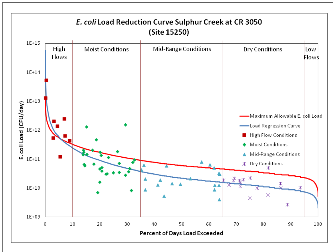
Figure 5.9 E. coli load duration curve for station 15250.
