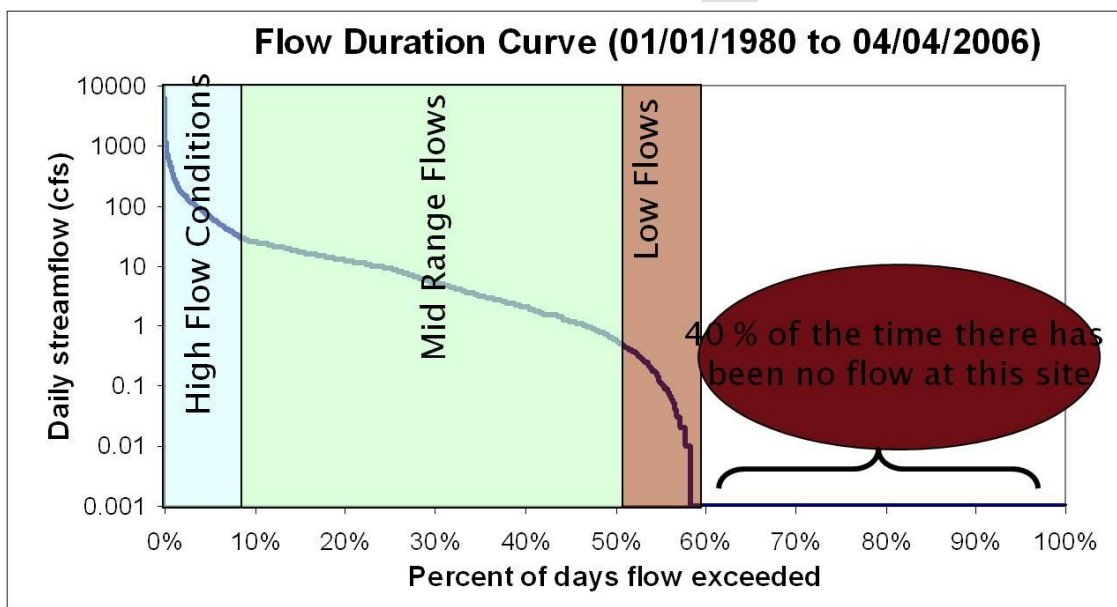
Figure 4.2 Example of a flow duration curve.
