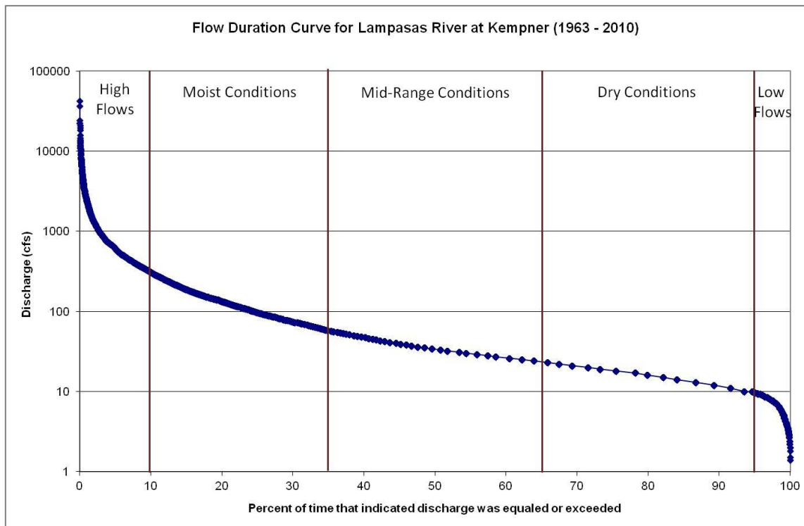
Figure C.1 Flow Duration Curve (FDC) for streamflow conditions at Station 11897 on the Lampasas River, near Kempner, Texas.
